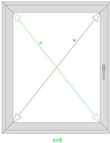
Fig. 10. Measuring diagonals:
