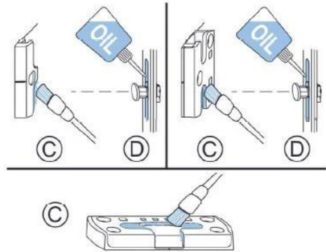
Lubrication points
