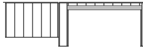
Wall Detail - 8
