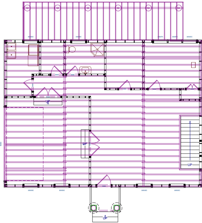
1st Floor
