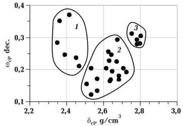
Fig. 3. Crossplot of hydrogen index vs density for determination of the type of clay minerals: 1 — montmorillonites, 2 — mixture of minerals, 3 — chlorites.
