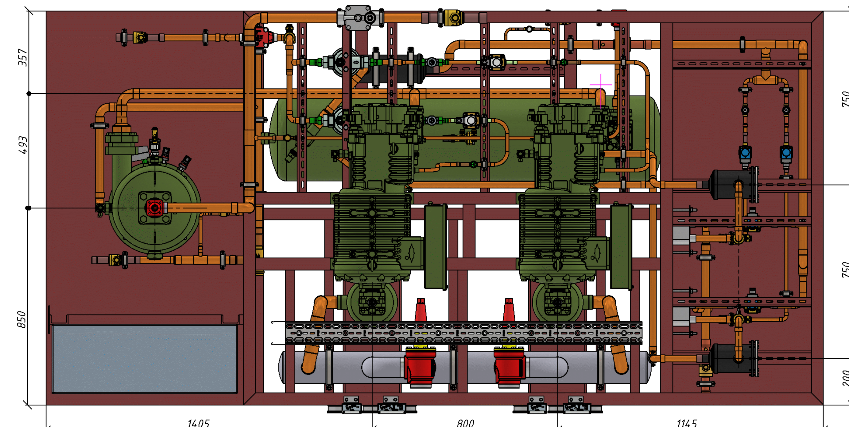
C (1:10)
