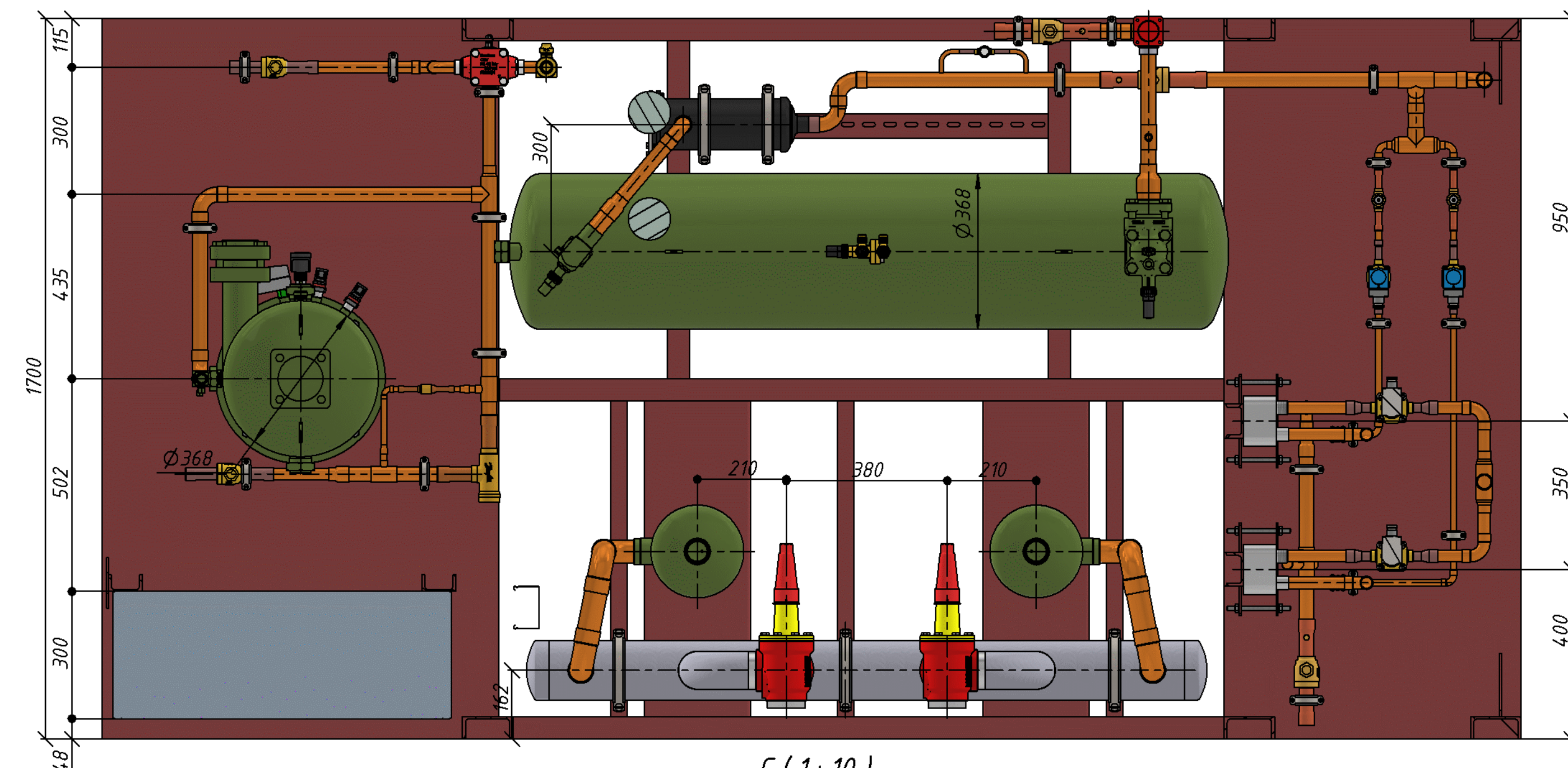
C (1:10)
