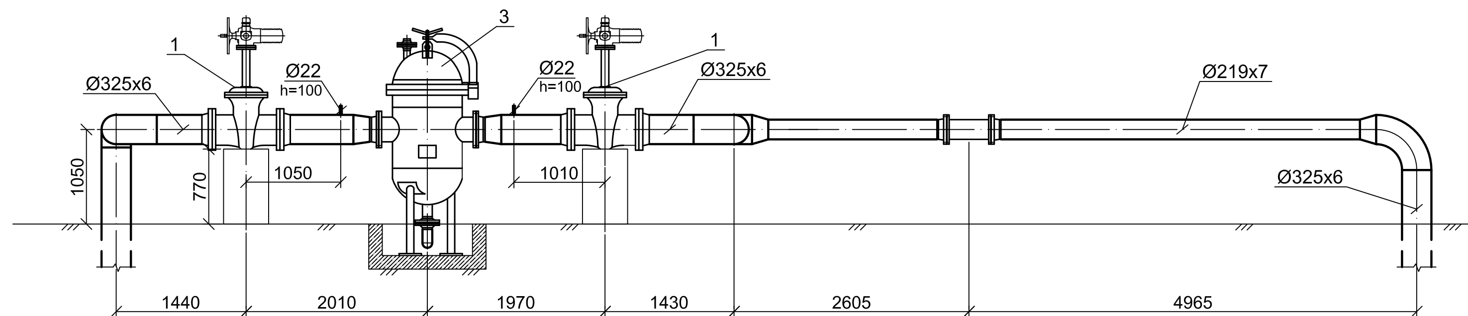
1-1 (1:50)
