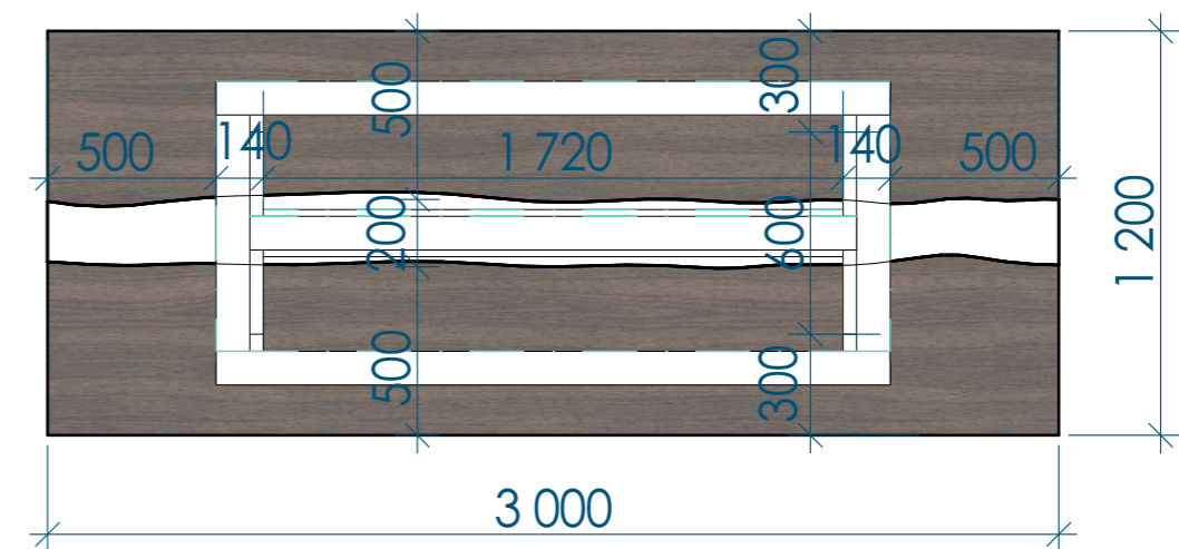
Top view
